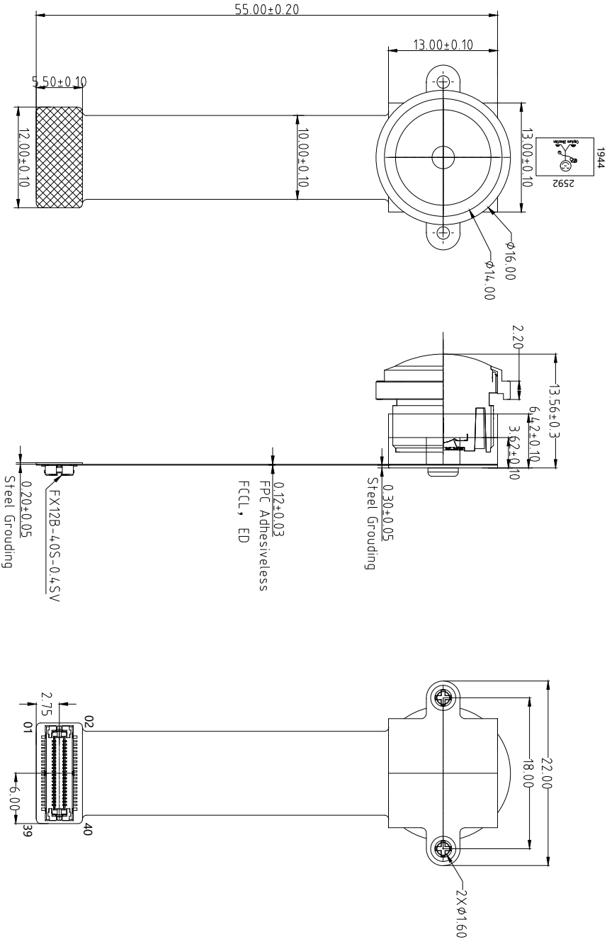
TOP VIEW
